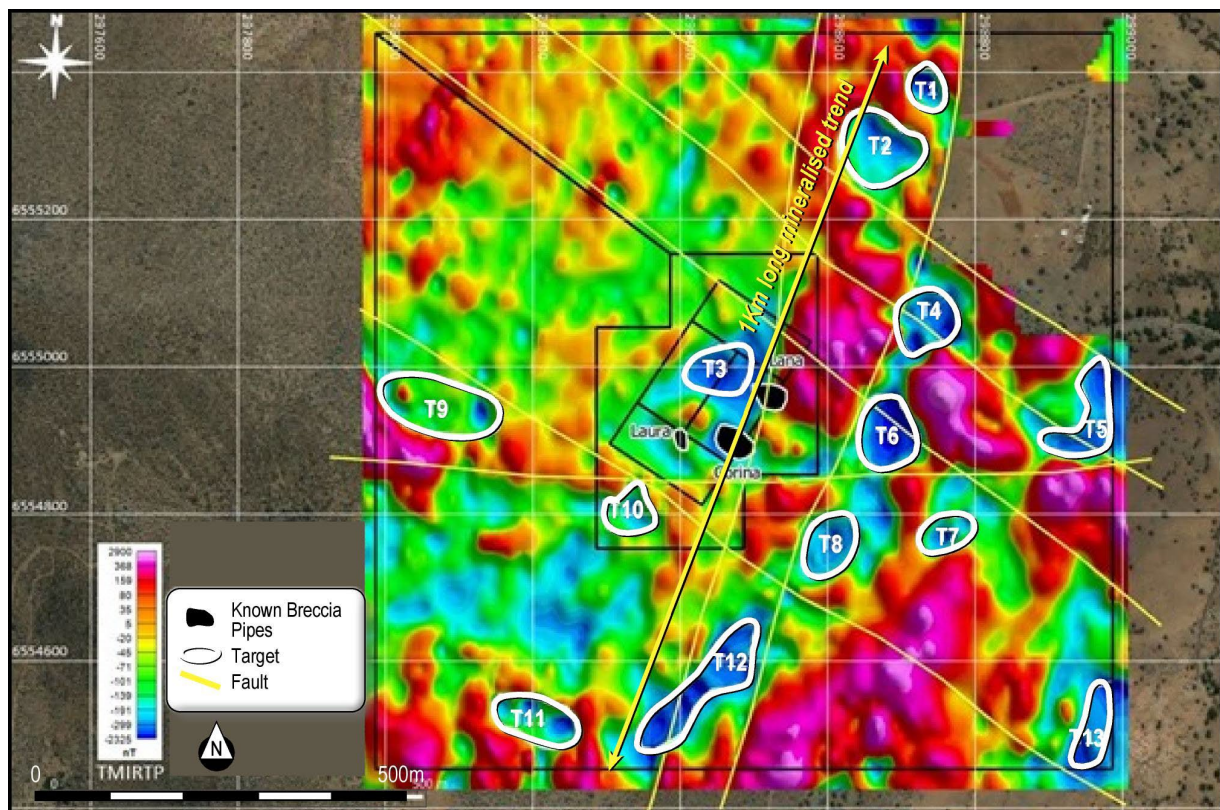
Figure 2: Plan view of high-resolution ground magnetic data (high pass TMIRTP), showing position of Lana Corina prospect and high priority targets identified from geophysical data (refer ASX announcement 18 May 2022).
