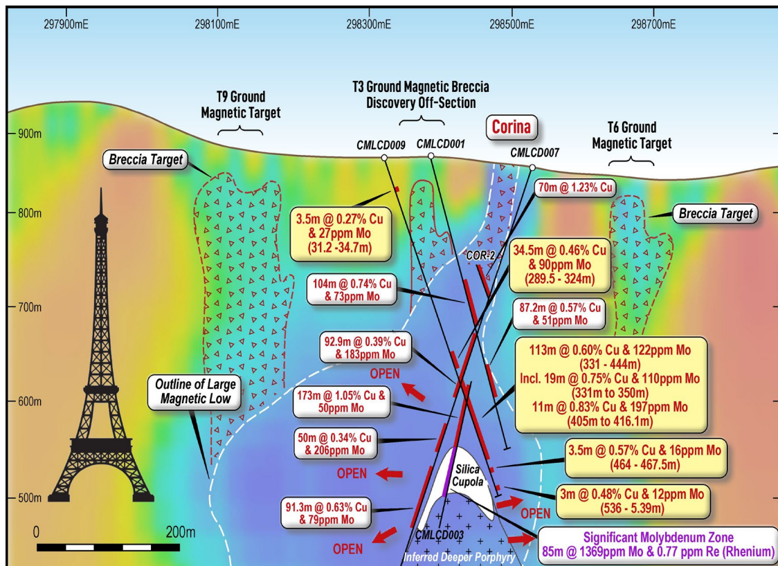
Figure 3: Schematic section looking north showing position of drillholes, geophysical targets and the high-grade Mo and Re mineralisation hosted within deeper silica rich cupola. (Refer ASX announcement 31 August 2022).
